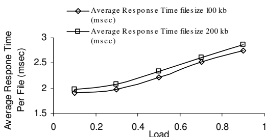
Fig. 18. Average response time versus load
