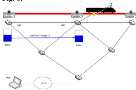
Fig. 8. Populating buffers across interconnected light-trails.
