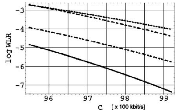
Figure 5. Packet loss ratio estimations, M1
